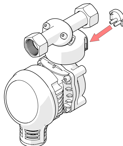
6. Insert the tightening key to lock the 360 connection in the installed position
