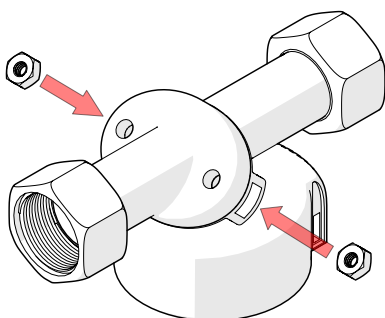
3. Insert the 2 nuts in the appropriate seats of the 360 connection
