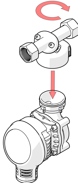
5. Insert and position the 360 connection in the desired position on the dosing pump
